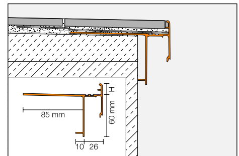
Assembly with Schlüter-DITRA and Schlüter-BARA-RAKEG
