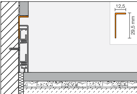
Shadow joint angle profile Schlüter®-DESIGNBASE-CQ/SG
