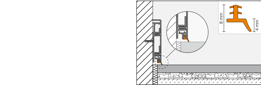
Sealing lip Schlüter®-DESIGNBASE-CQ/Z
